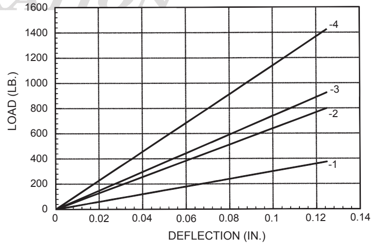
52545 COMPRESSION LOAD VS DEFLECTION
