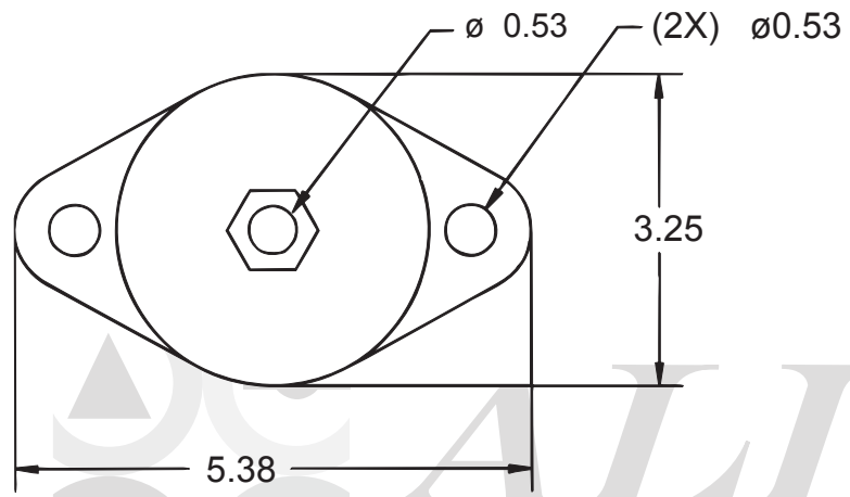
52545- ( ) RETAINER FOR STANDARD NUT OR BOLT
