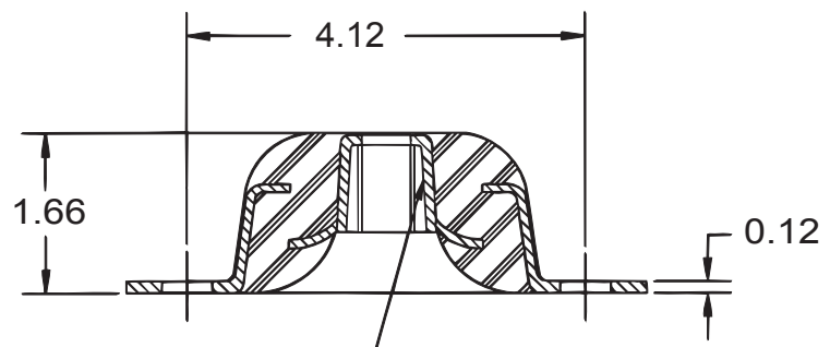
52545- ( ) RETAINER FOR STANDARD NUT OR BOLT
